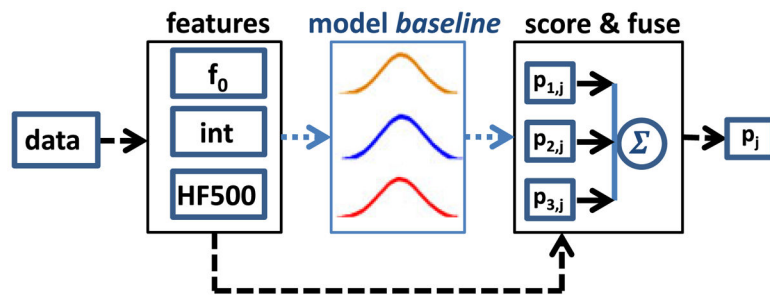
Fig. 1. Arousal rating flow diagram. Utterance j is first transformed into three feature streams. Each feature produces an arousal score based on a baseline model trained for each individual. Lastly, the scores are combined into a final arousal rating, p_j .
