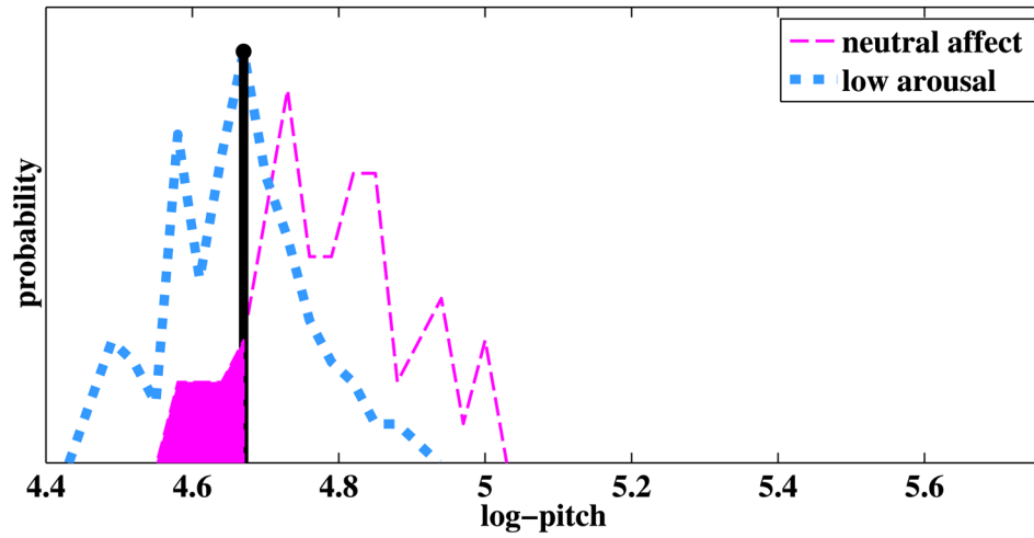
Fig. 3. Arousal rating of a token with labeled low arousal having a log-pitch of 4.67. The filled-in portion represents the fraction of neutral samples which are lower than 4.67.
